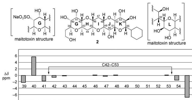
Figure 1. Differences in the ^{13}\text{C} chemical shift ( \Delta\delta /ppm) between GHIJK fragment 2 and the values reported for maitotoxin ( 1 ) in the same solvent system. ^{13}\text{C} chemical shifts of 2 [150 MHz, 1:1 [\text{D}_4]\text{methanol}/[\text{D}_5]\text{pyridine} (reported values for maitotoxin in parentheses)] [19] : C-39: 74.5 (72.3), C-40: 73.2 (78.9), C-41: 70.3 (68.5), C-42: 81.2 (80.6), C-43: 69.8 (69.6), C-44: 36.3 (36.3), C-45: 77.8 (77.7), C-46: 77.4 (77.5), C-47: 37.7 (37.4), C-48: 67.7 (67.8), C-49: 85.8 (85.8), C-50: 70.1 (70.1), C-51: 74.9 (74.9), C-52: 72.1 (72.1), C-53: 79.3 (79.4), C-54: 71.3 (69.8), C-55: 85.0 (78.2).
